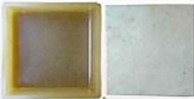
POWER - 07 - 10X10 Paver Area=0.69 Sq.Ft. For 100 Sq.Ft.=144 Nos
