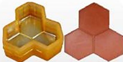
POWER - 32 - Trihex Area=0.277 Sq.Ft. For 100 Sq.Ft.=360 Nos
